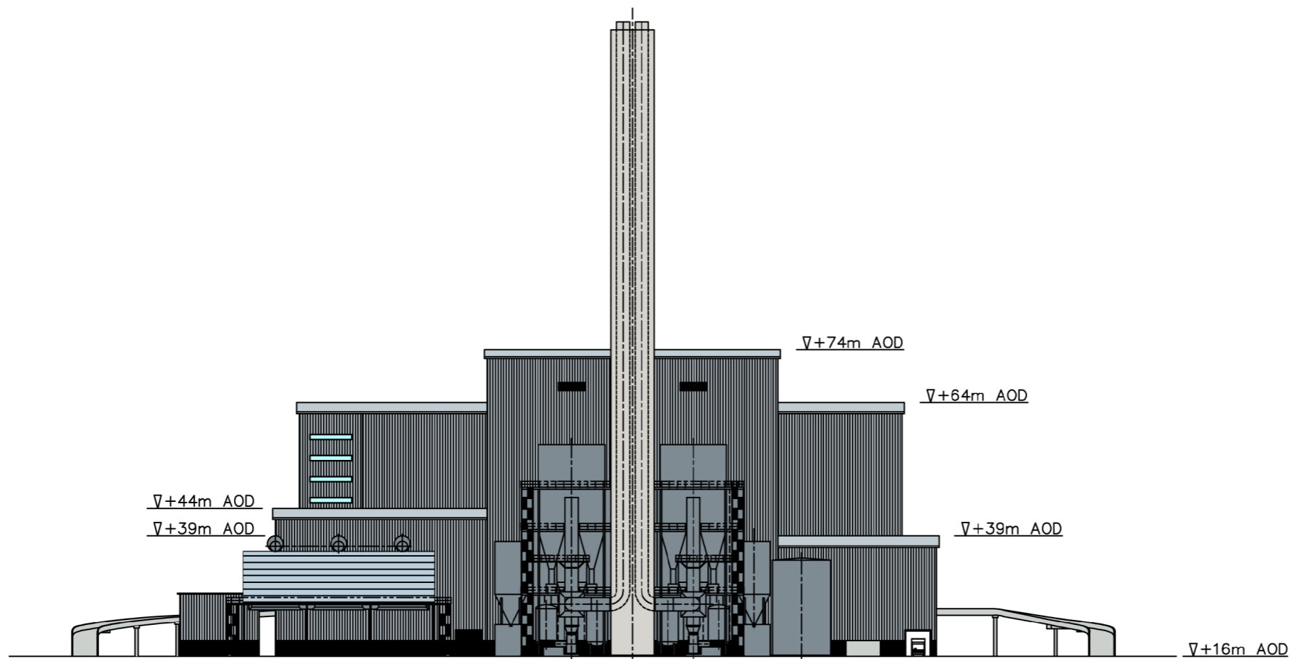
Vertical Boiler
