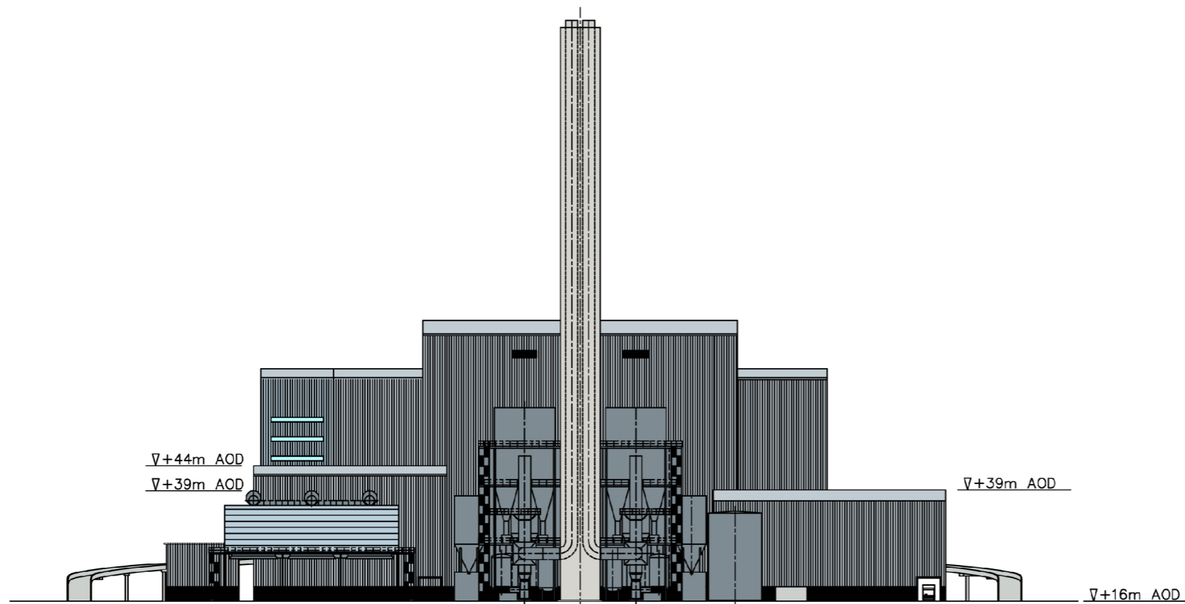
Horizontal Boiler
