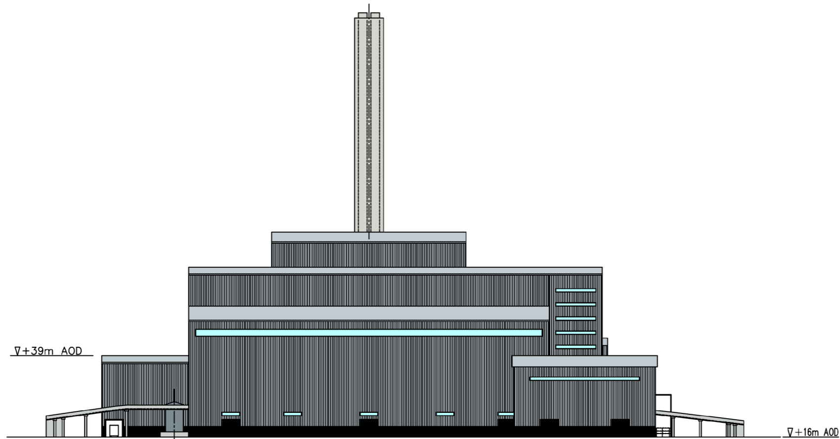
Horizontal Boiler
