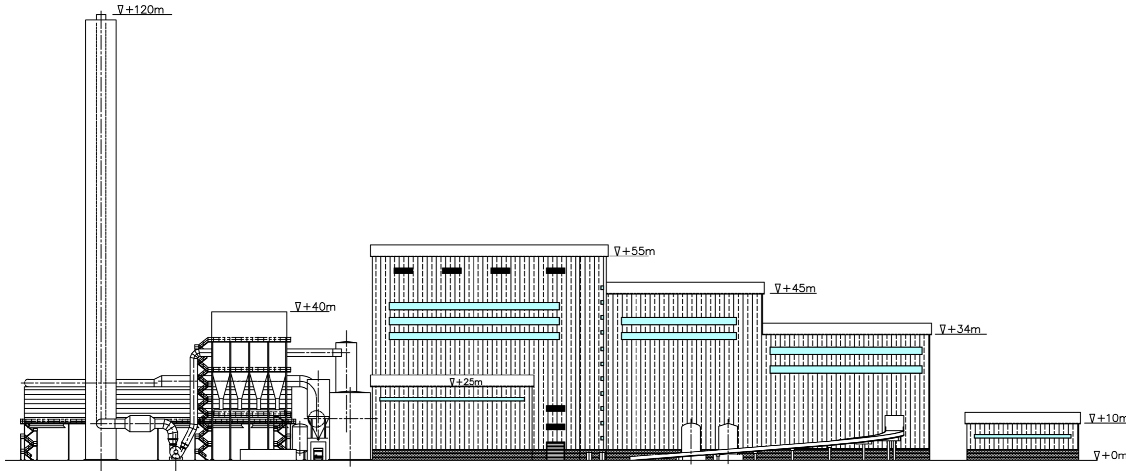
Horizontal Boiler
